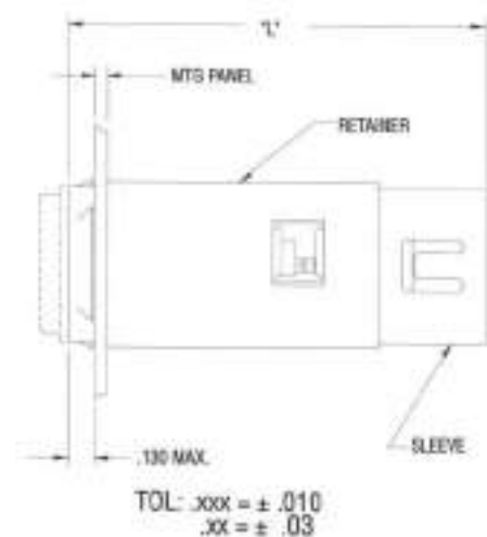
Snap-On Mounting Sleeve
