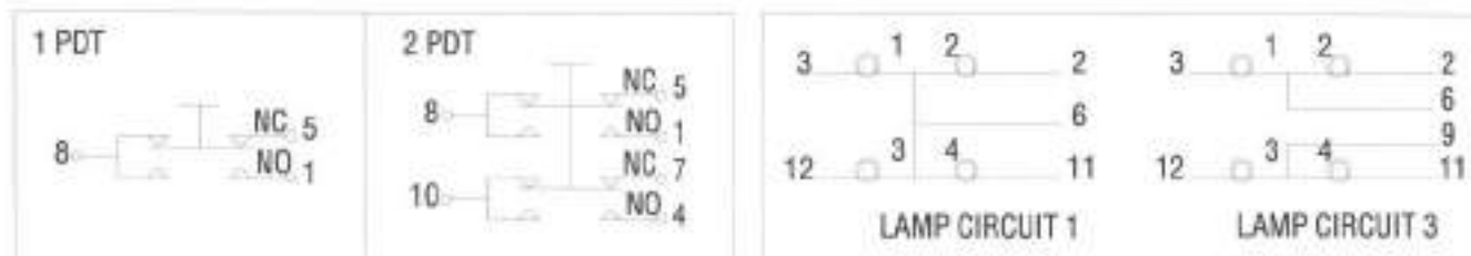
Form "C" Switch Circuits
